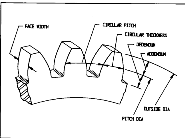
Figure 2 - Common terms used in defining gears.
