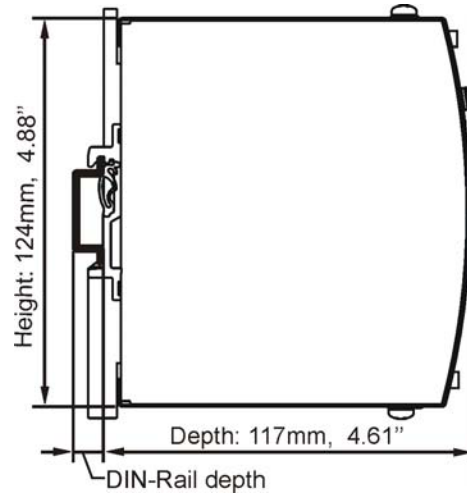
Fig. 22-2 Side view
