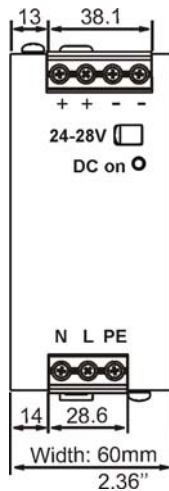
Fig. 22-1 Front view
