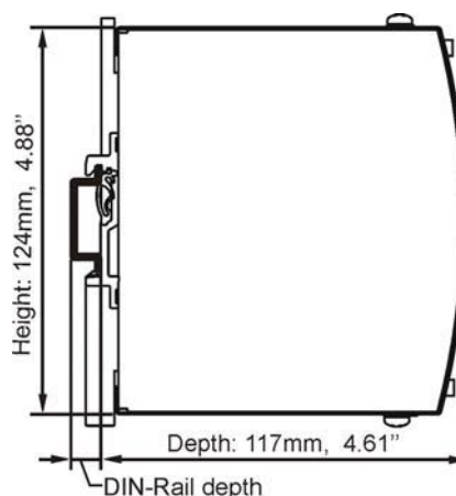
Fig. 23-2 Side view
