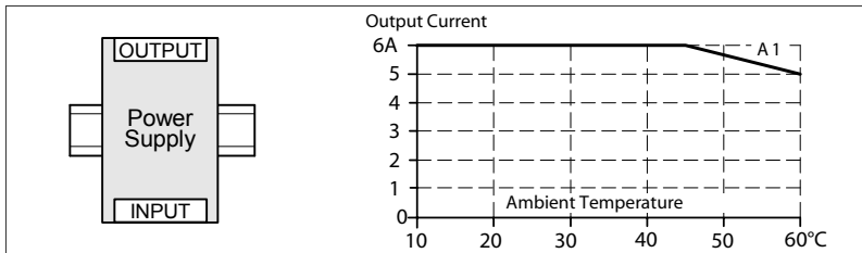
Fig. 26-7 Mounting Orientation A Standard Orientation
