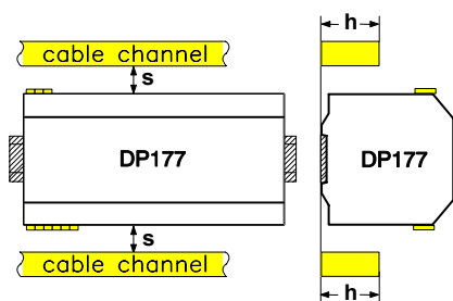
Required mounting dimensions
