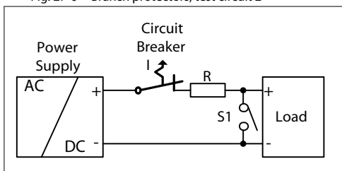
Fig. 27-6 Branch protectors, test circuit 2
