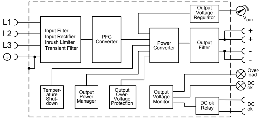
Fig. 12-1 Functional diagram
