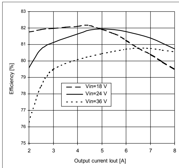
Efficiency (typ.)
