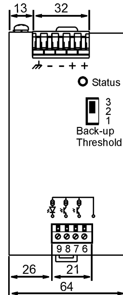
Fig. 20-2 Front view
