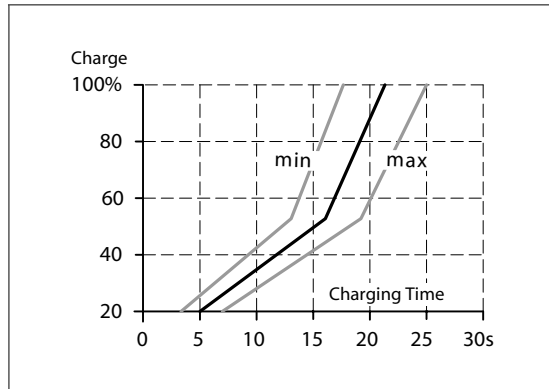
Fig. 6-1 Buffer charging time, 48V
