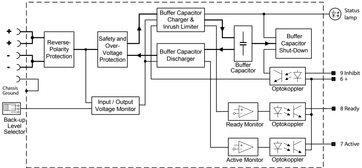
Fig. 8-1 Functional diagram
