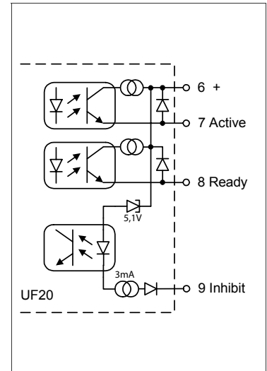
Fig. 10-2 Signals schematic
