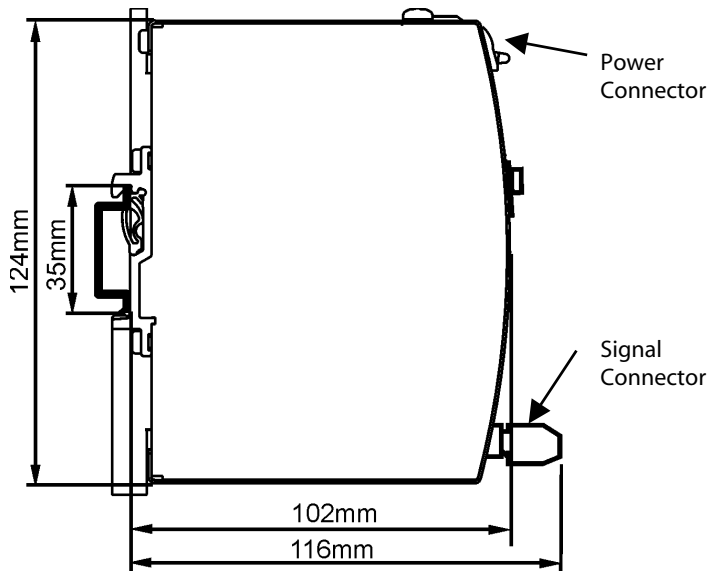
Fig. 20-1 Side view
