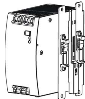
Fig. 3-5 DIN-Rail Mount
